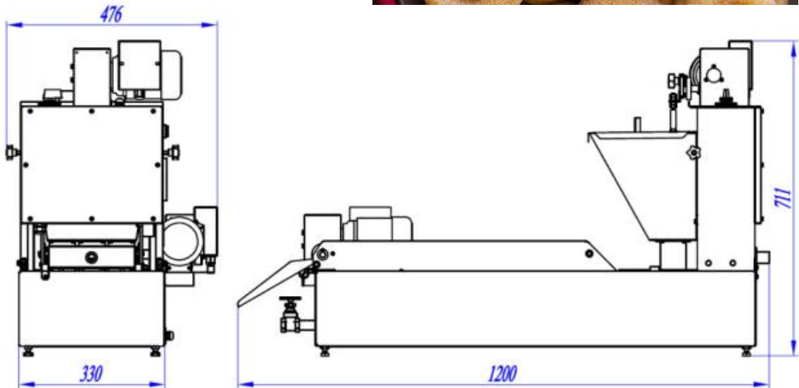
Dimensions of Both MP2 and MP3 (in mm)
